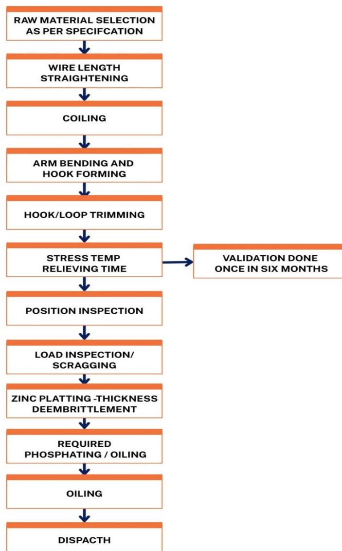
GENERIC PROCESS FLOW CHART FOR TENSION AND TORSION SPRINGS
